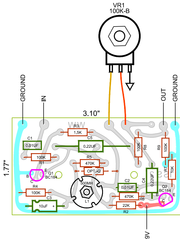
UNKNOWN VERSION OF COLORSOUND "WAH WAH" PCB LAYOUT BY PAUL MAROSSY 2/15/18
